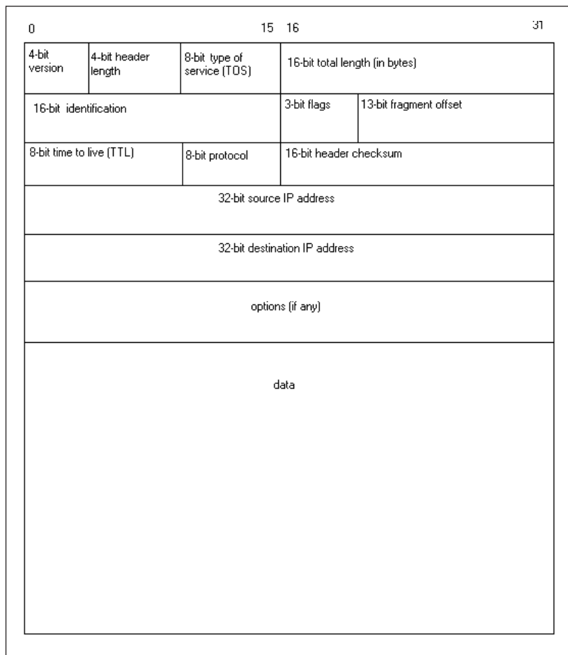
Figure 5-1: IP header
